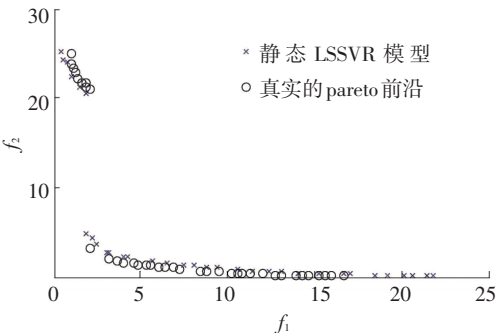
图 4 静态 LSSVR 模型与真实函数的 Pareto 前沿 Fig.4 The Pareto front obtained from one time LSSVR and actual Pareto front
